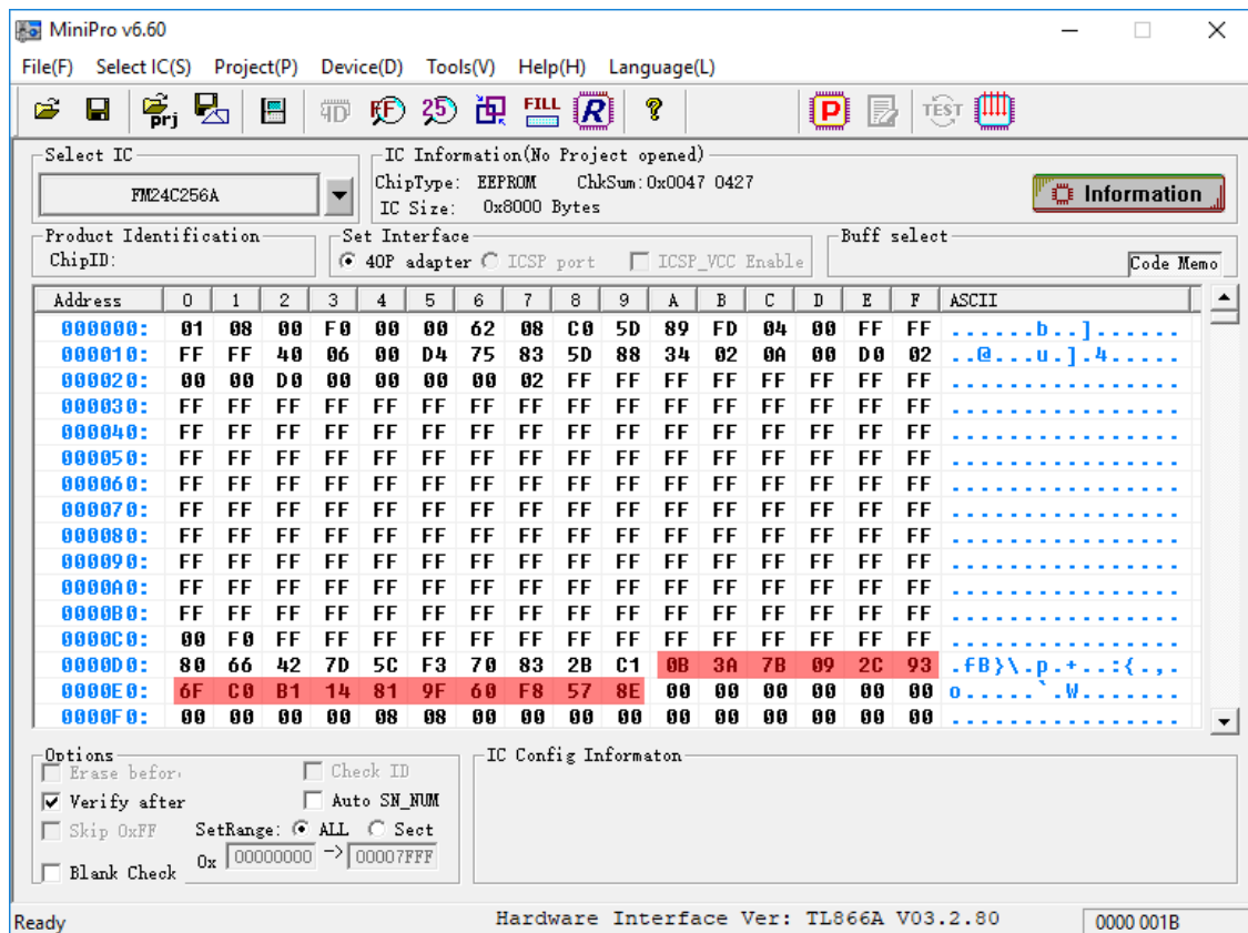
Figure 7: Memory dump of the EEPROM chip containing the Bluetooth link key of the paired device
