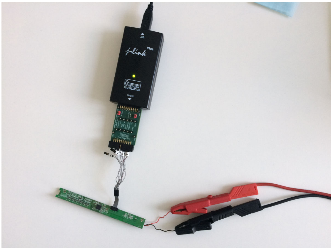
Figure 8: SWD (Serial Wire Debug) connection to Microsoft keyboard using Segger J-Link Pro
