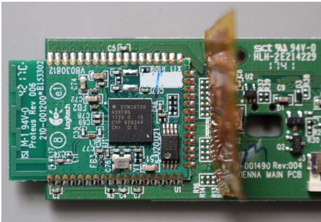
Figure 5: PCB of the tested wireless keyboard Logitech K480 with CYW20730 Bluetooth transceiver and EEPROM chip
