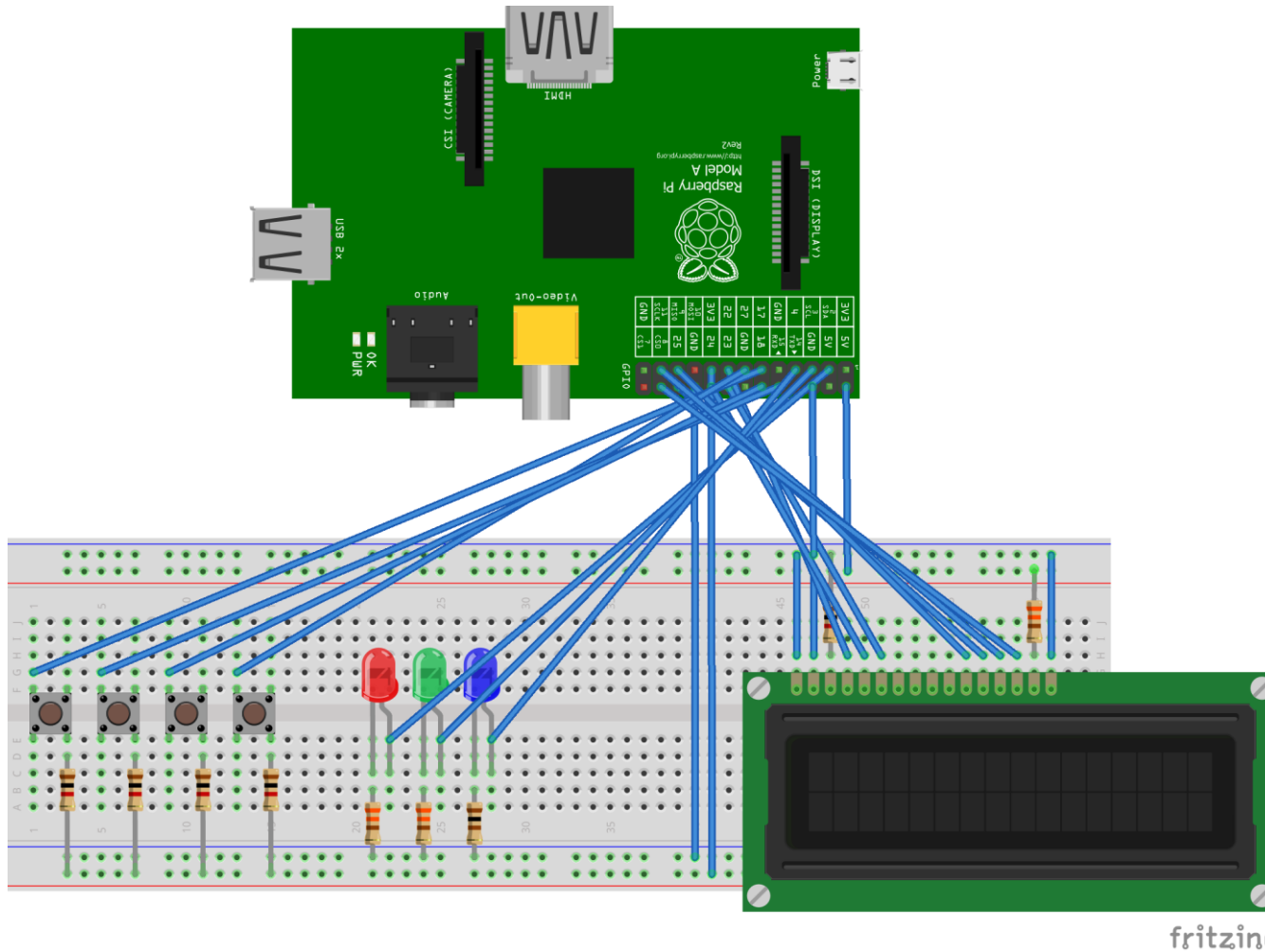
Breadboard setup for a very simple Raspberry Pi shield (Radio Hack Box Prototype)
