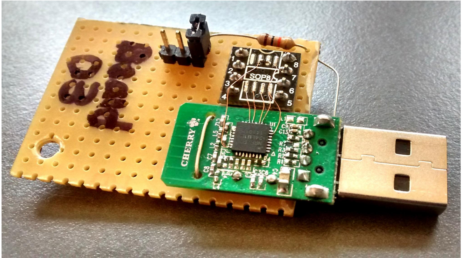
SPI read and write access to a Cherry USB dongle (thanks to Alexander Straßheim)
