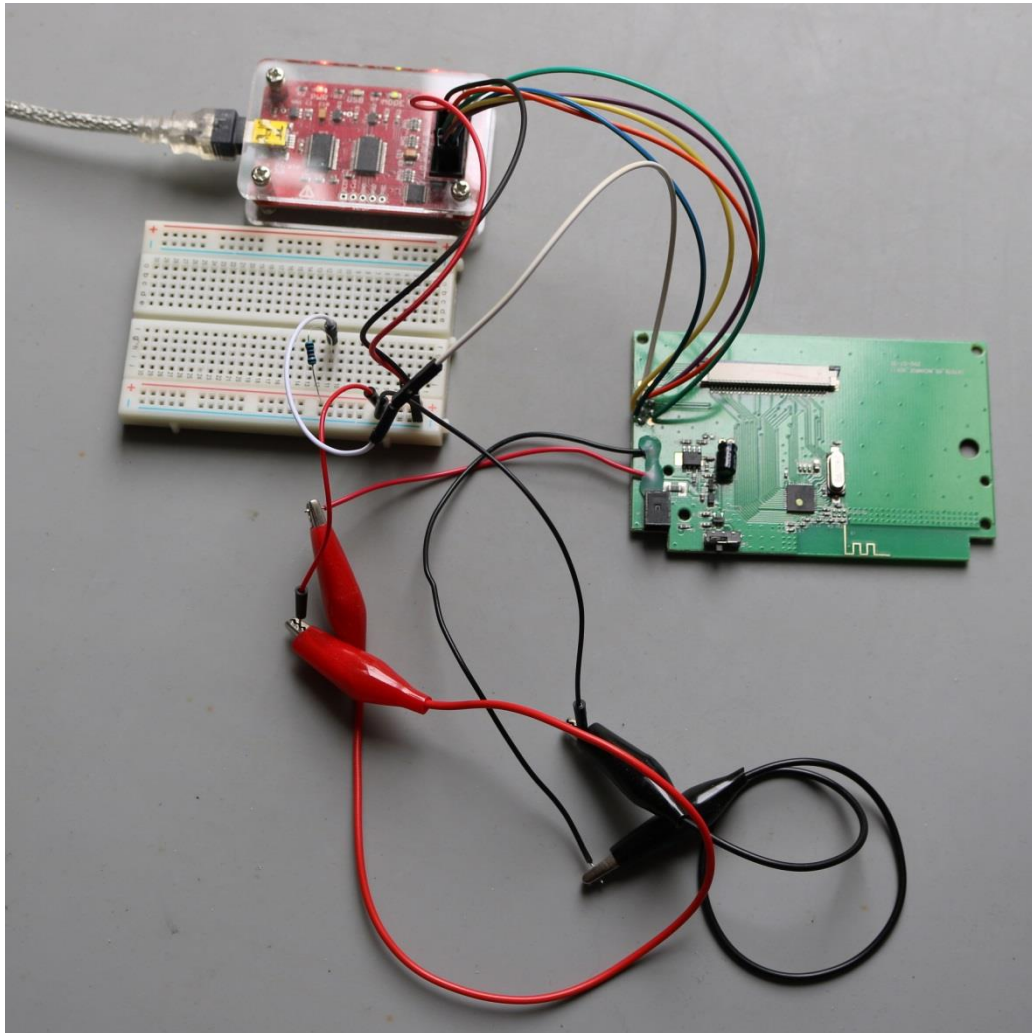
SPI read and write access to a Cherry wireless keyboard
