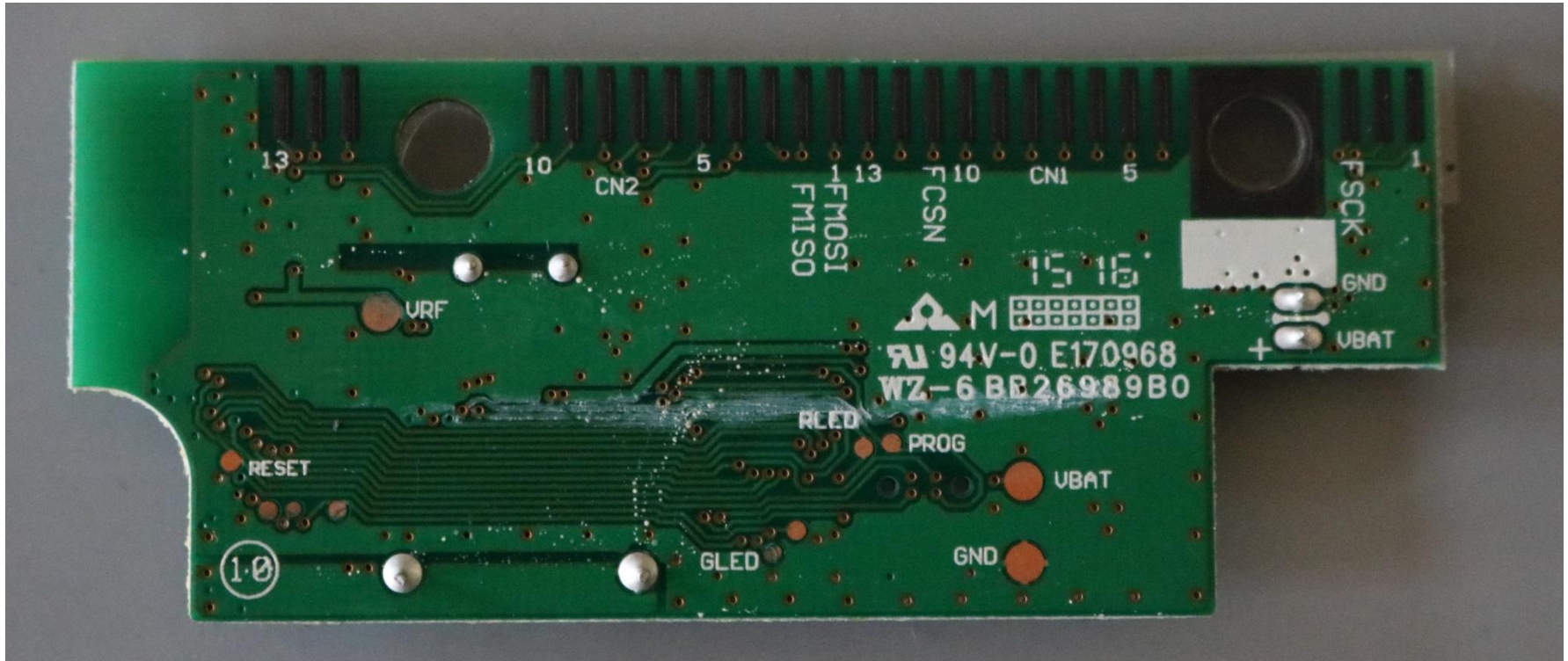
PCB back side of a Microsoft wireless keyboard
